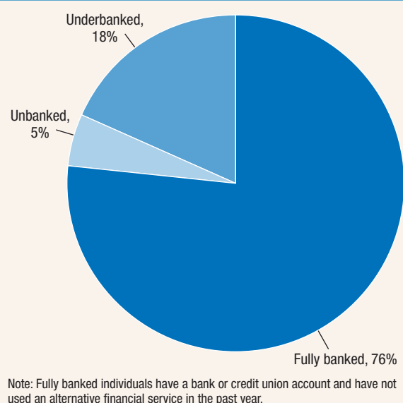
Figure 15. Banking status
